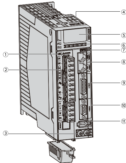
Figure 2-2 Servo drive components
